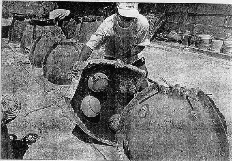
ABOVE: Larry Beggs pulls the mold off a Reef Ball as Harry Rolfe works on other molds in the background. The balls are made of a special concrete that is poured into molds made out of fiberglass and inflatable balls. Ben Gray/Staff
